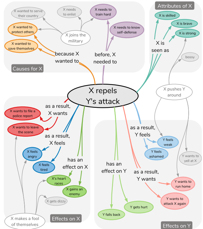
Figure 1: A tiny subset of ATOMIC, an atlas of machine commonsense for everyday events, causes, and effects.
